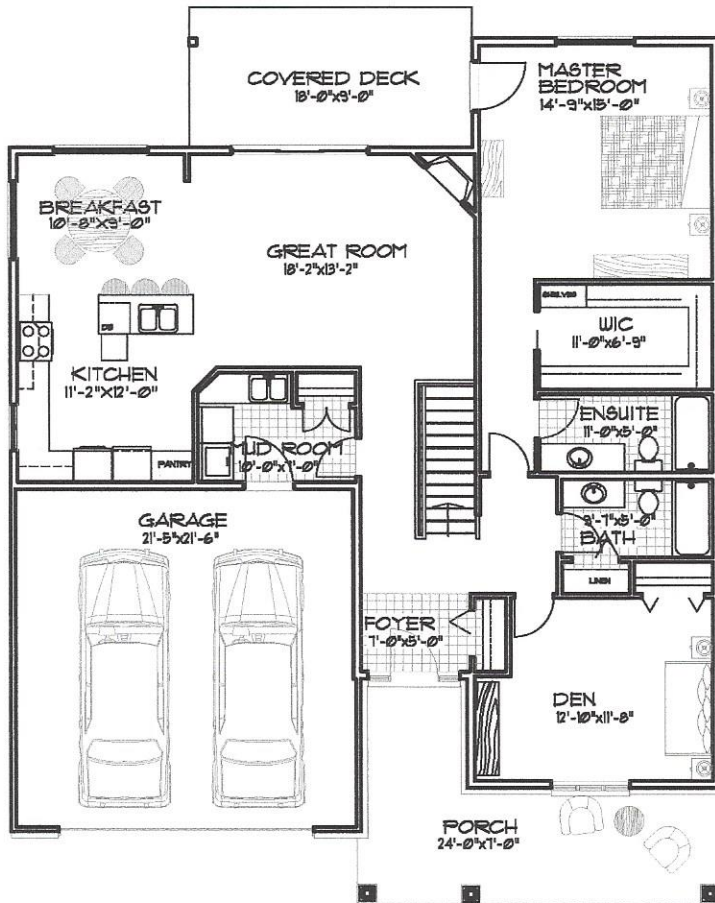
Ground Floor Plan 45'-2" x 55'-6"
