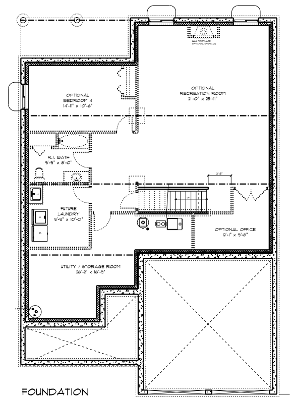
FOUNDATION 41'-0" x 60'-3"
