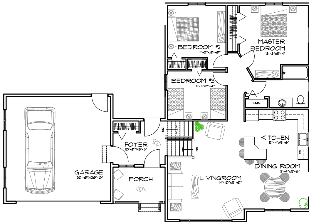
Ground Floor Plan 59'-0" x 42'-0"
