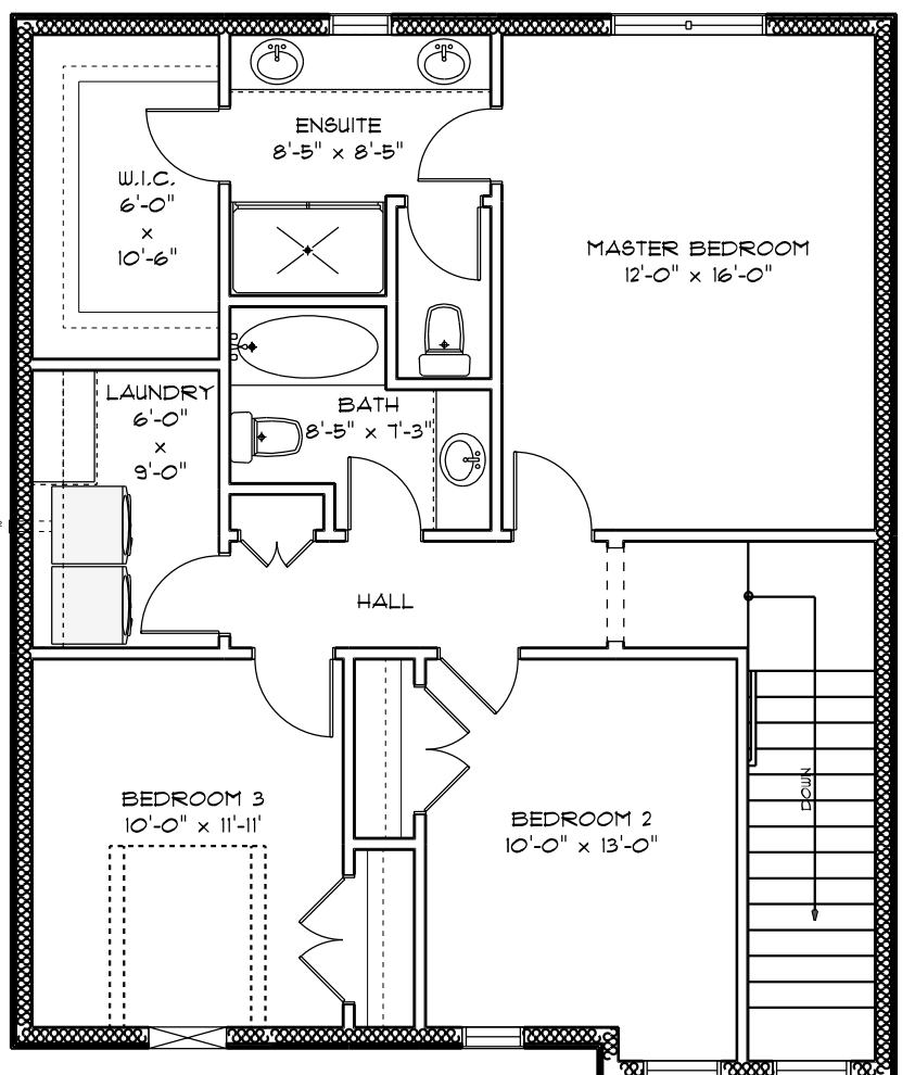
SECOND FLOOR LIVING AREA = 959.0 SQ. FT.
