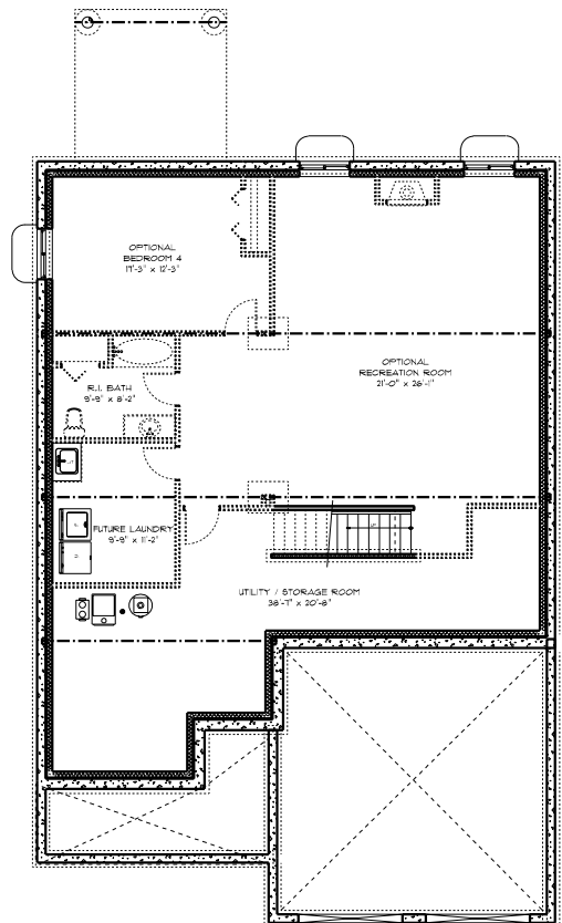
FOUNDATION 41'-0" x 60'-3"
