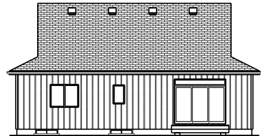
REAR ELEVATION
