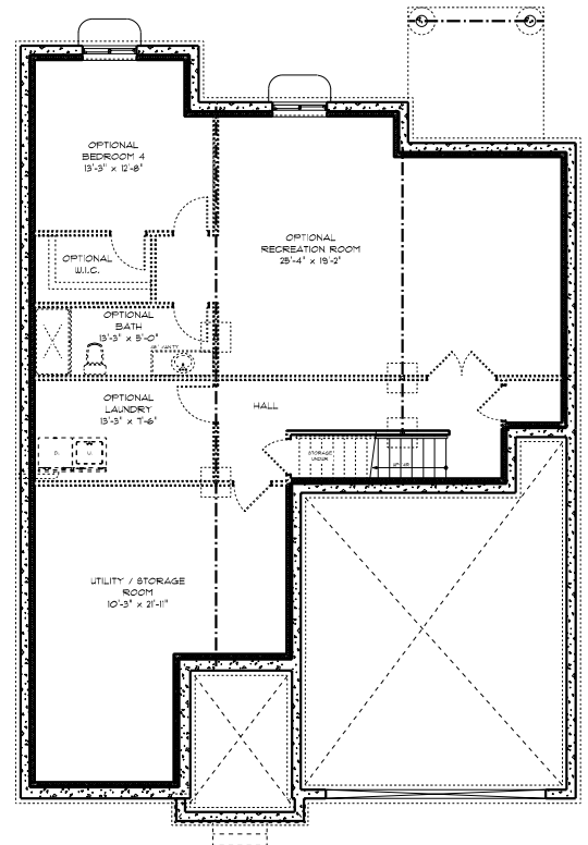
FOUNDATION PLAN 41'-0" x 51'-3"
