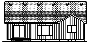
REAR ELEVATION
