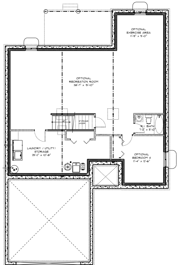
FOUNDATION 41'-0" x 64'-0"
