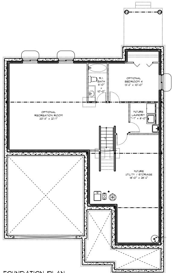
FOUNDATION PLAN 41'-6" x 58'-8"
