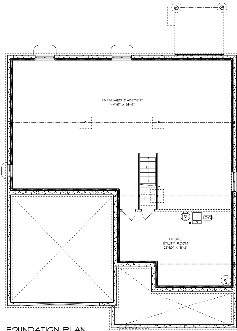
FOUNDATION PLAN 46'-9" x 55'-6"
