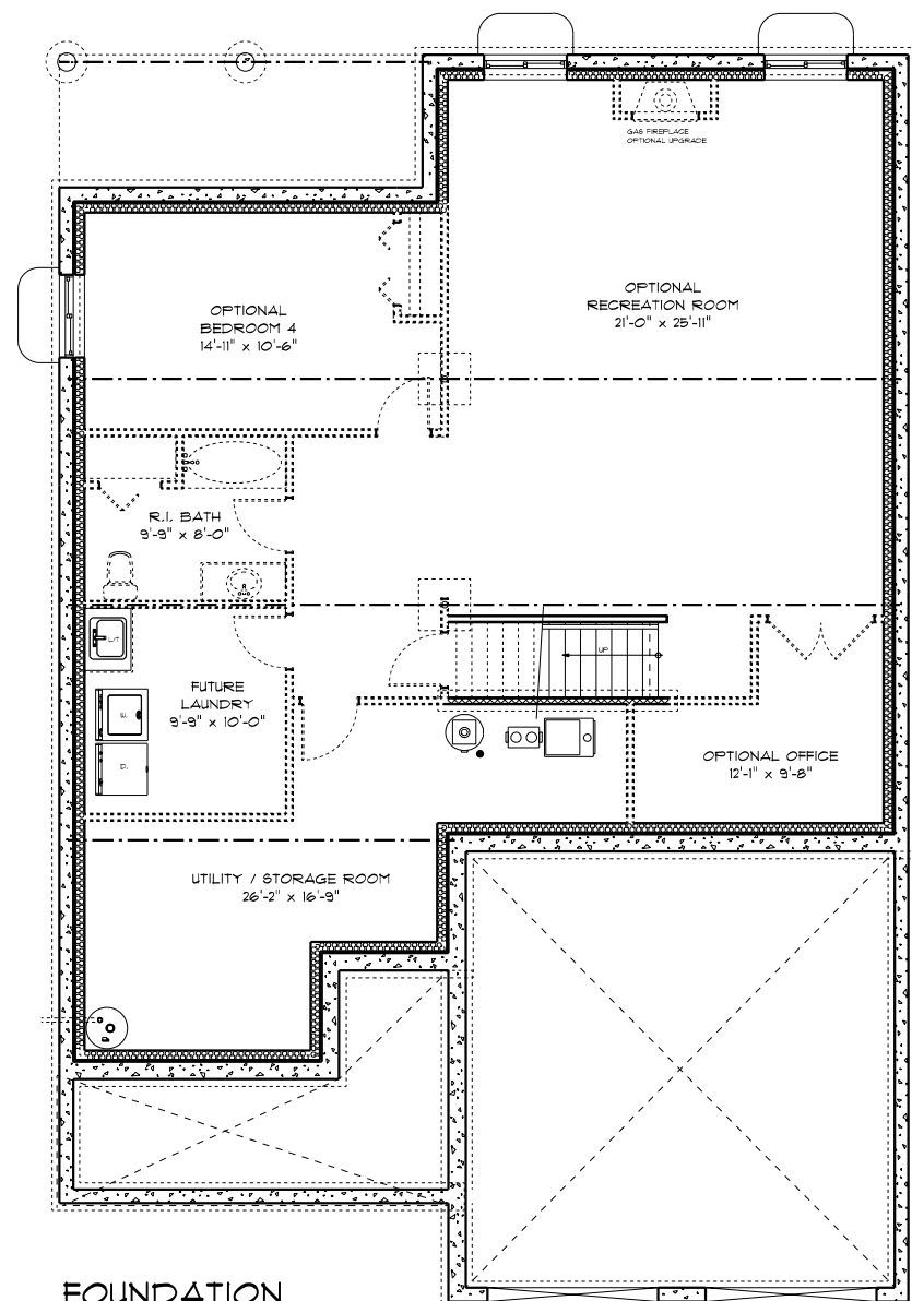
FOUNDATION 41'-0" x 60'-3"
