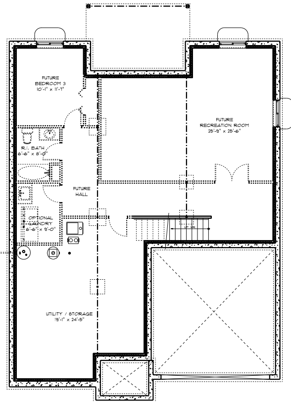
FOUNDATION PLAN 40'-7" x 53'-9"
