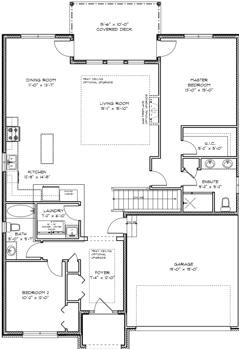
MAIN FLOOR PLAN TOTAL LIVING AREA = 1,612.2 SQ. FT. TOTAL GARAGE AREA = 382.1 SQ. FT.
