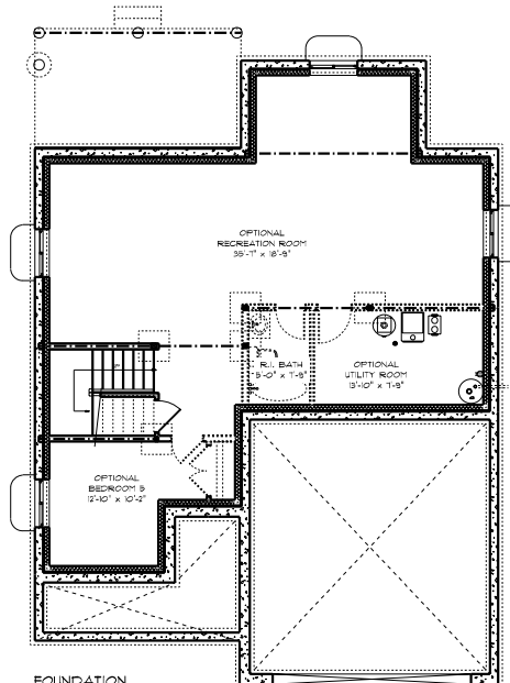
FOUNDATION 38'-0" x 51'-1"
