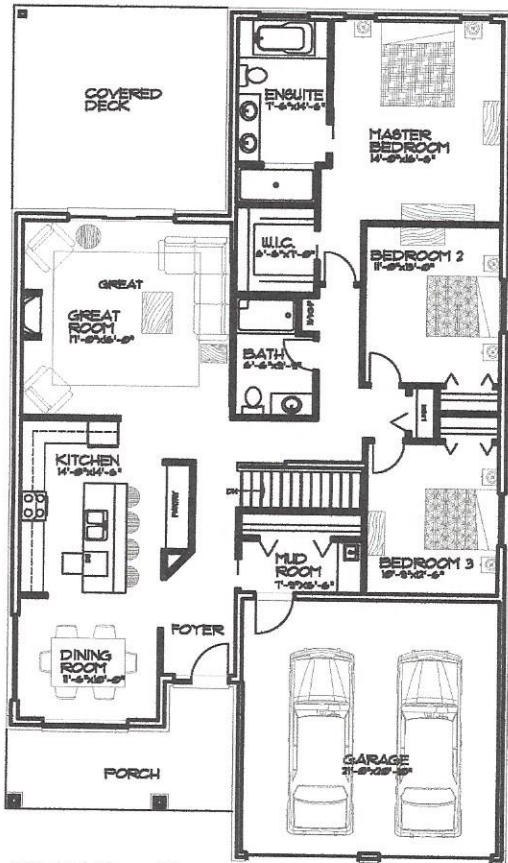
Ground Floor Plan 41'-0" x 10'-3"
