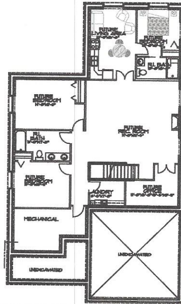
Basement Plan
