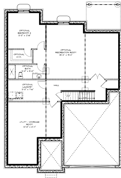
FOUNDATION PLAN 41'-0" x 51'-3"
