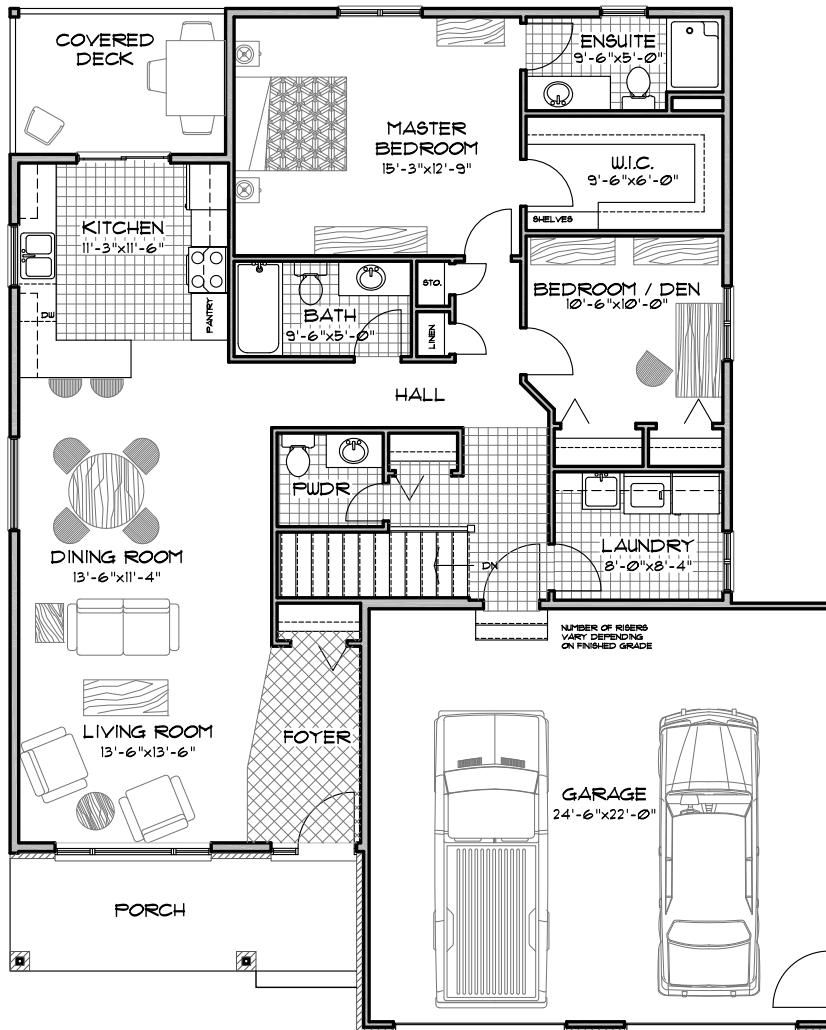
Ground Floor Plan 44'-0" x 54'-9"
