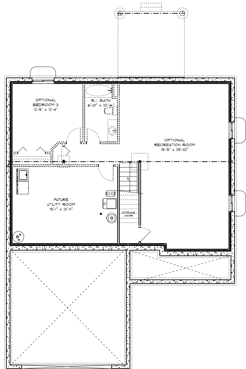
FOUNDATION PLAN
